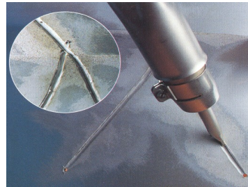
Tack Welding
