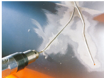
Drilling ends of cracks to relieve stress in the part
